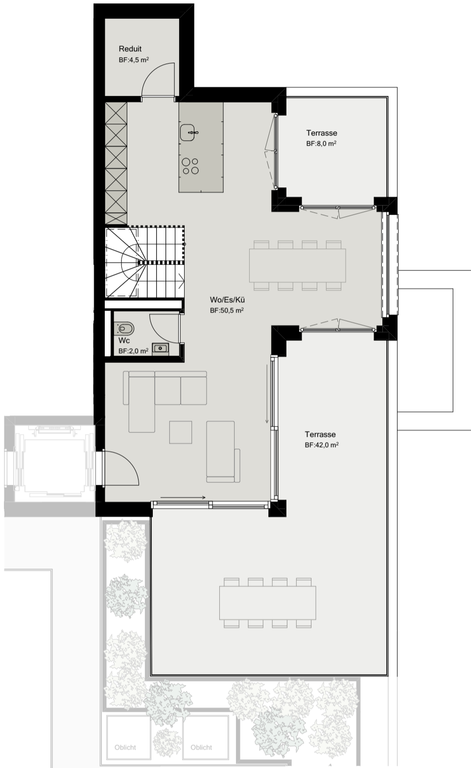
Attikageschoss
