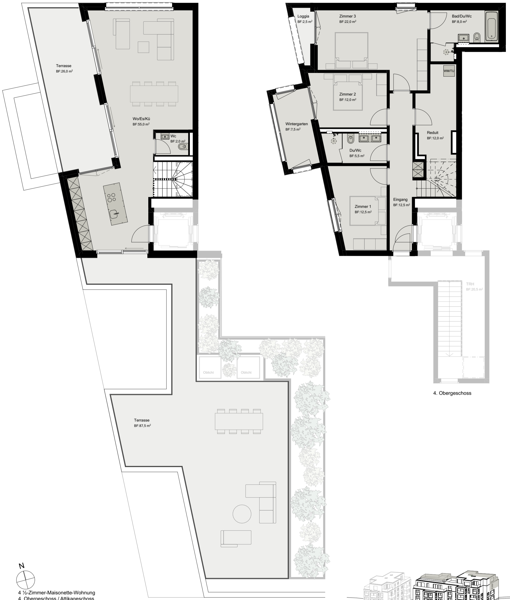
Attikageschoss
